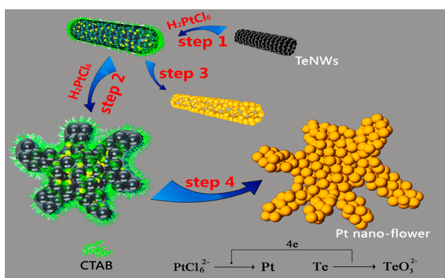
Figure 2. Simulation of mechanism of galvanic replacement from TeNWs to Pt nanoflowers with the equivalent charge reaction process.
